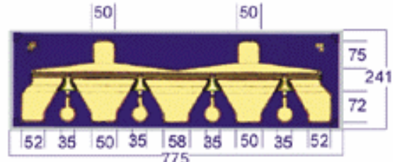
Chip Dimensions: 775 x 241 microns Chip Thickness: 100 microns
