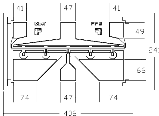
Chip Dimensions: 406 x 241 microns Chip Thickness: 100 microns
