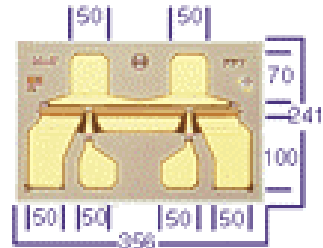
Chip Dimensions: 356 x 241 microns Chip Thickness: 100 microns
