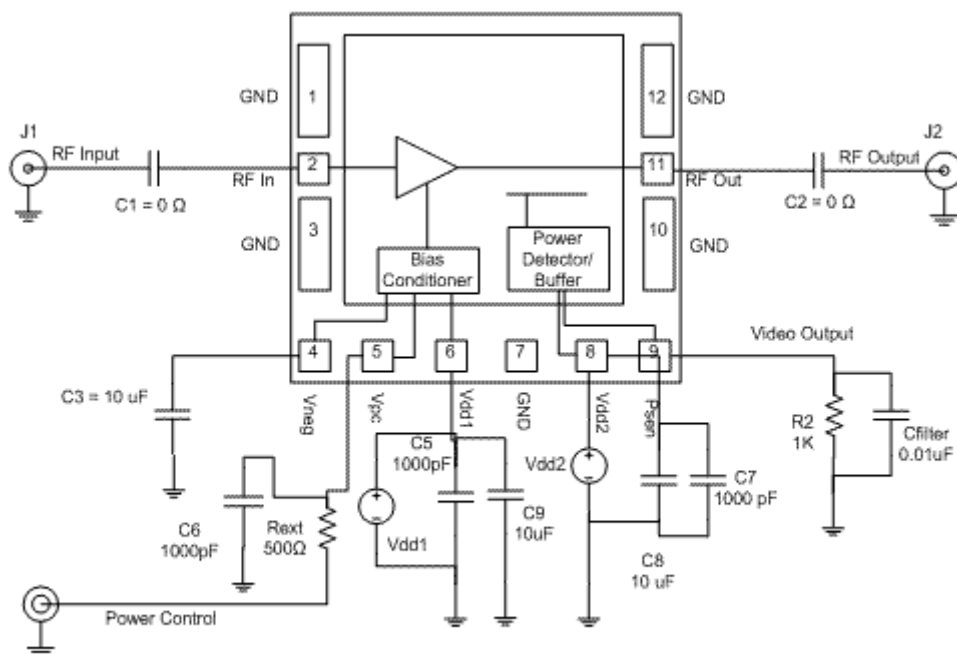
Figure 4 Evaluation Board Schematic
