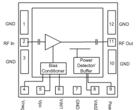
Figure 3 Block Diagram
