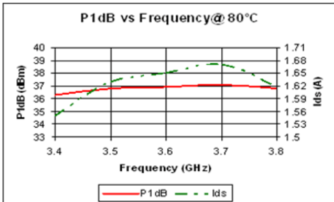
Figure 7 P1dB
