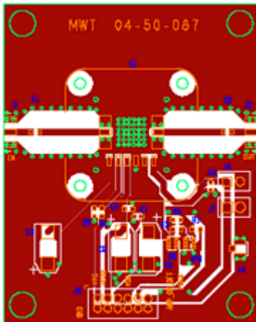
Figure 1 Evaluation Board
