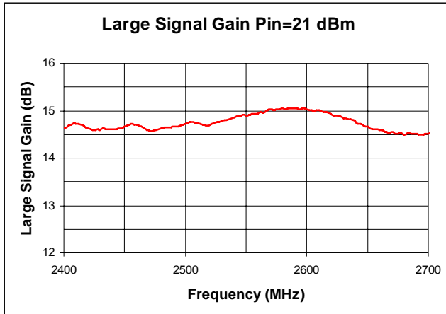
Figure 4 Gain Response
