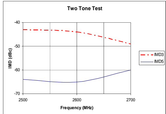
Figure 5 OIP3
