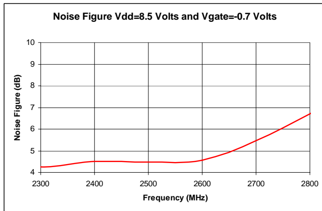
Figure 2 Noise Figure
