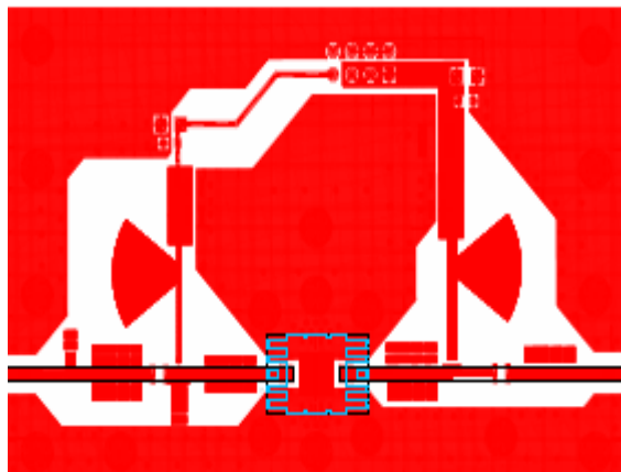
Figure 1 Evaluation board
