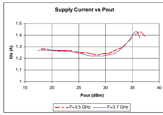
Figure 3 Supply Current
