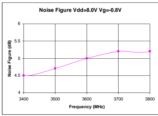
Figure 2 Noise Figure
