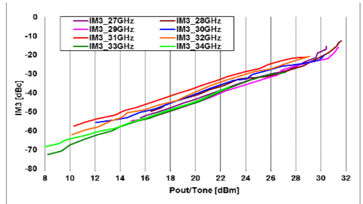
IM3 Level [dBc] vs. output power/toner [dBm] @Vds=6V, Idsq=2.8A
