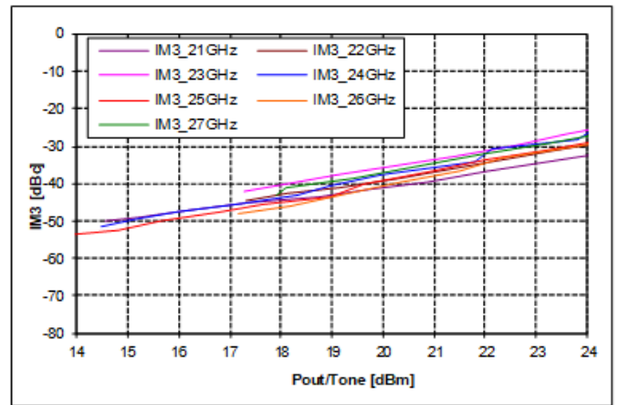
IM3 Level vs. single tone output power [dBm/tonne]
