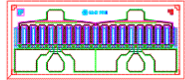
Chip Dimensions: 775 x 343 microns Chip Thickness: 100 microns
