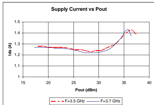
Figure 3 Supply Current
