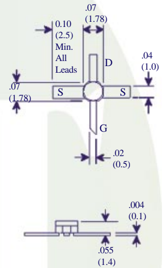
Package 73 (Epoxy Seal)
