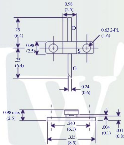
Package 71 (Solder Seal)
