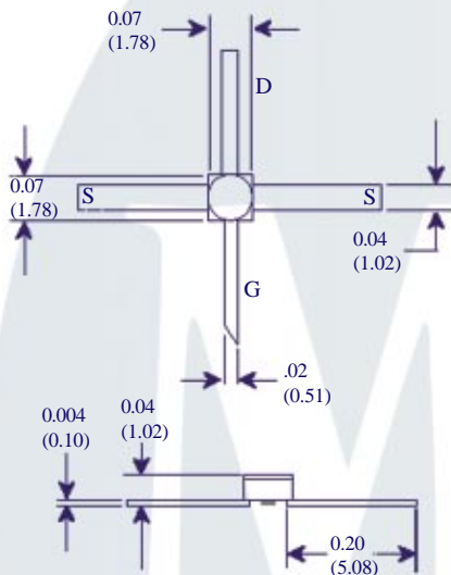
Package 70 (Solder Seal)
